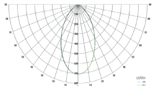
Polar Candela Distribution Plot Using Missed Rays
