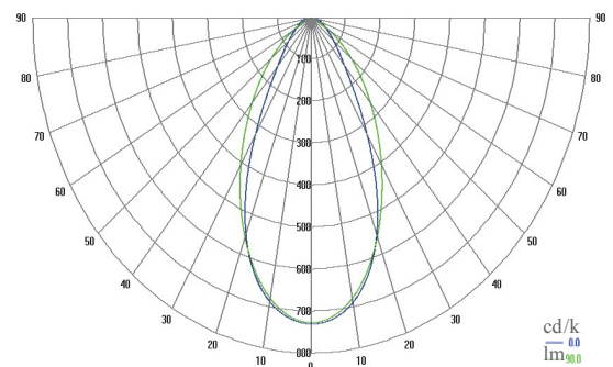
Polar Candela Distribution Plot Using Missed Rays
