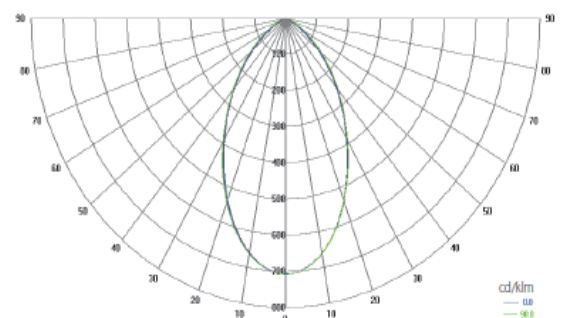
Polar Candela Distribution Plot Using Missed Rays
